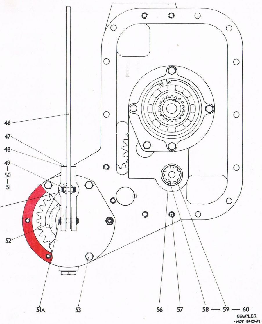
FIG. B SANDWICH GEARBOX (2400 SERIES) MF 165 & 178
