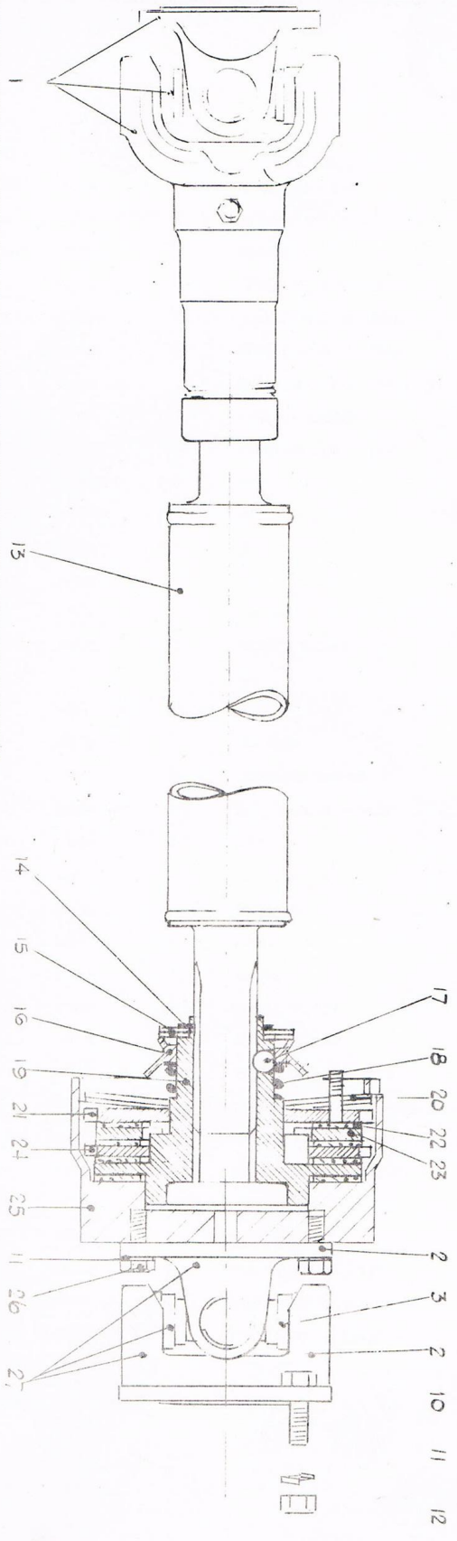
FIG. 5 DRIVE SHAFT / TORQUE CLUTCH
